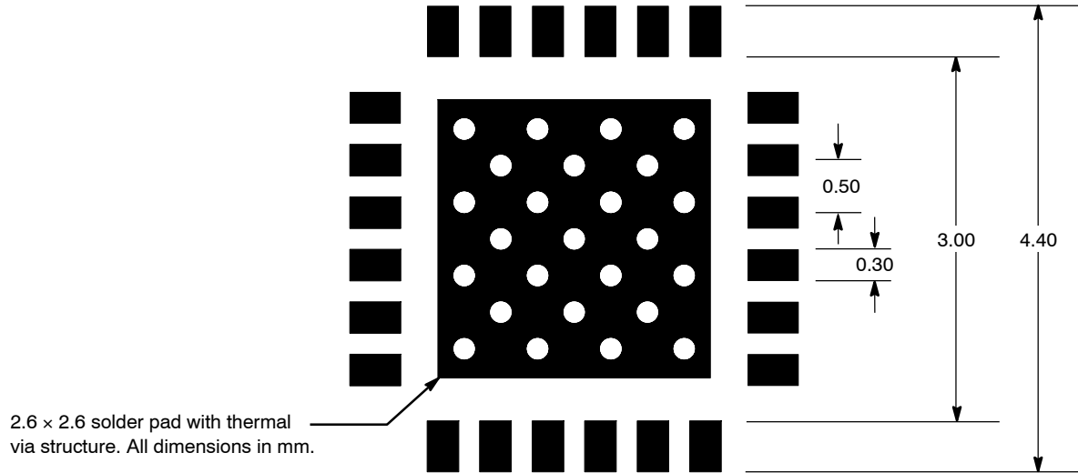
Figure 17. PCB Pad Layout for 24-Lead QFN 4 × 4
