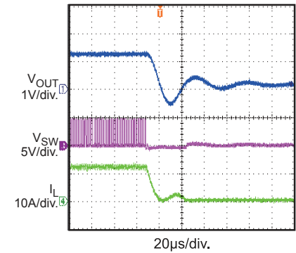
Thermal Shutdown
