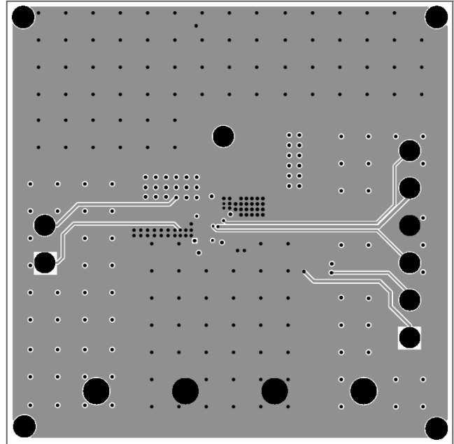
Figure 4: Inner Layer2
