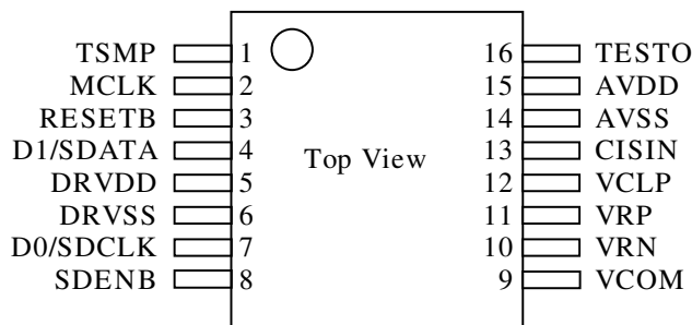
Fig. 2 Pin Allocation
