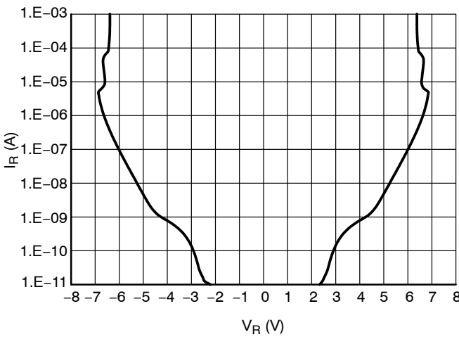
Figure 7. Breakdown Voltage
