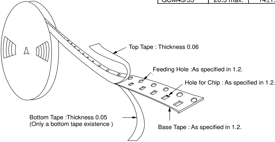
Fig.3 Taping Diagram
