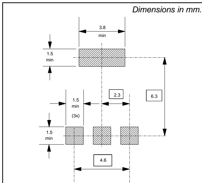
Fig.21. Soldering pattern for surface mounting.
