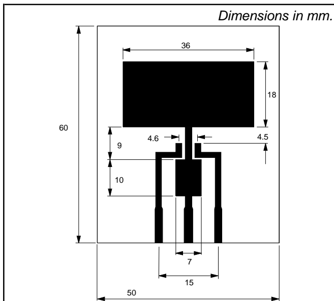
Fig.22. PCB for thermal resistance and power rating. PCB: FR4 epoxy glass (1.6 mm thick), copper laminate (35 μm thick).
