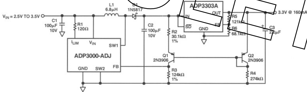
Figure 25. Constant Dropout Post Regulator
