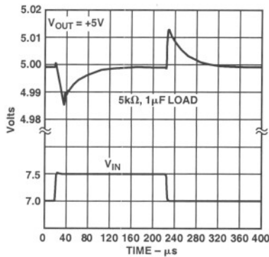
Figure 12. Line Transient Response
