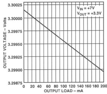
Figure 3. Output Voltage vs. Load Current
