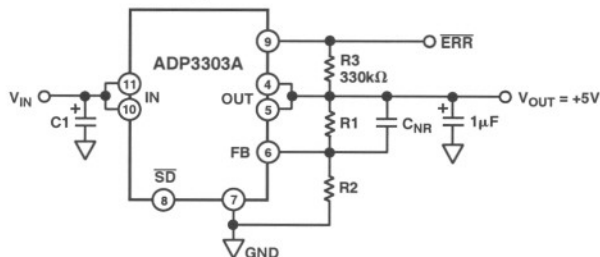
Figure 21. Noise Reduction Circuit
