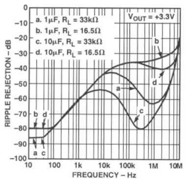
Figure 18. Power Supply Ripple Rejection
