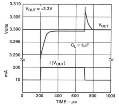
Figure 13. Load Transient for 10 mA to 200 mA Pulse
