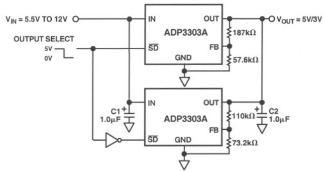
Figure 23. Crossover Switch
