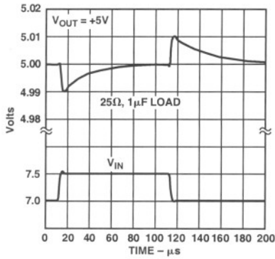
Figure 11. Line Transient Response
