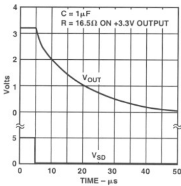
Figure 17. Turn Off
