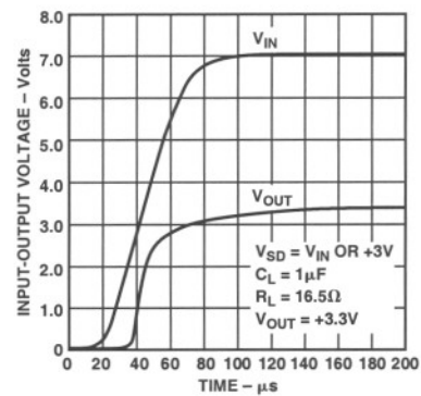
Figure 10. Power-Up Transient
