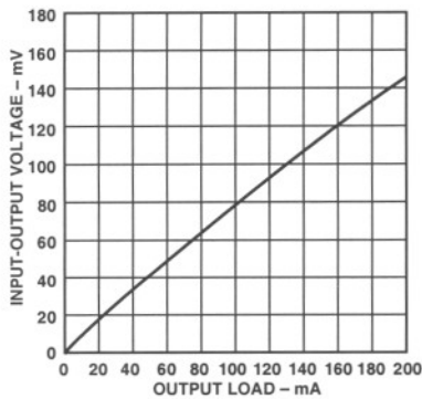
Figure 8. Dropout Voltage vs. Output Current
