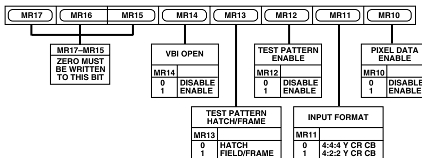
Figure 51. Mode Register 1
