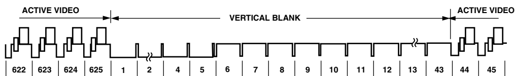
Figure 68. ITU-R.BT1358 (625p)
