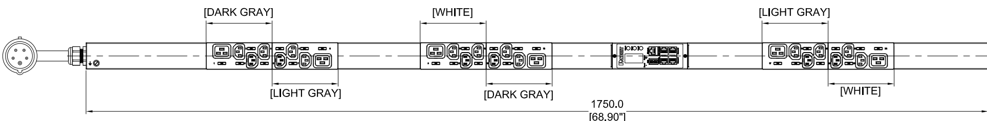
FRONT VIEW
