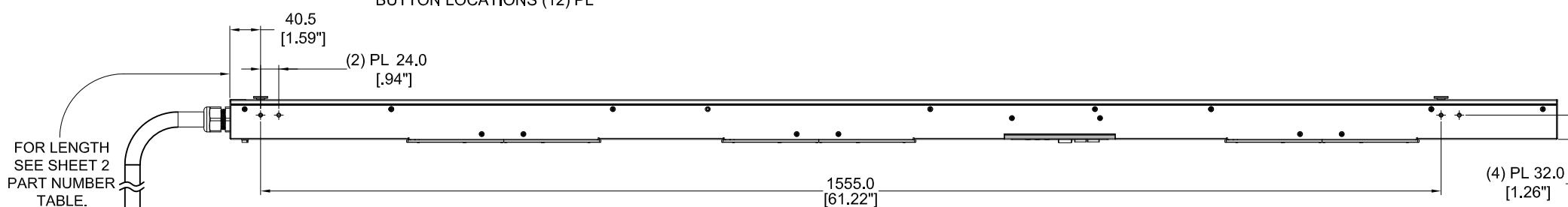
REAR VIEW
