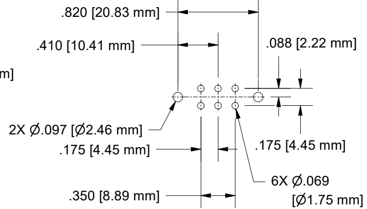
RECOMMENDED PCB FOOT PRINT (TOP VIEW)
