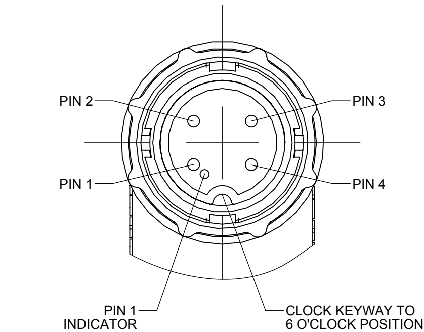
PIN CALLOUT VIEW FROM MATING SIDE OF CONNECTOR SCALE=3:1
