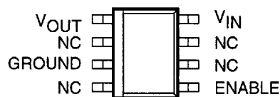
MIC5201-xxBM
