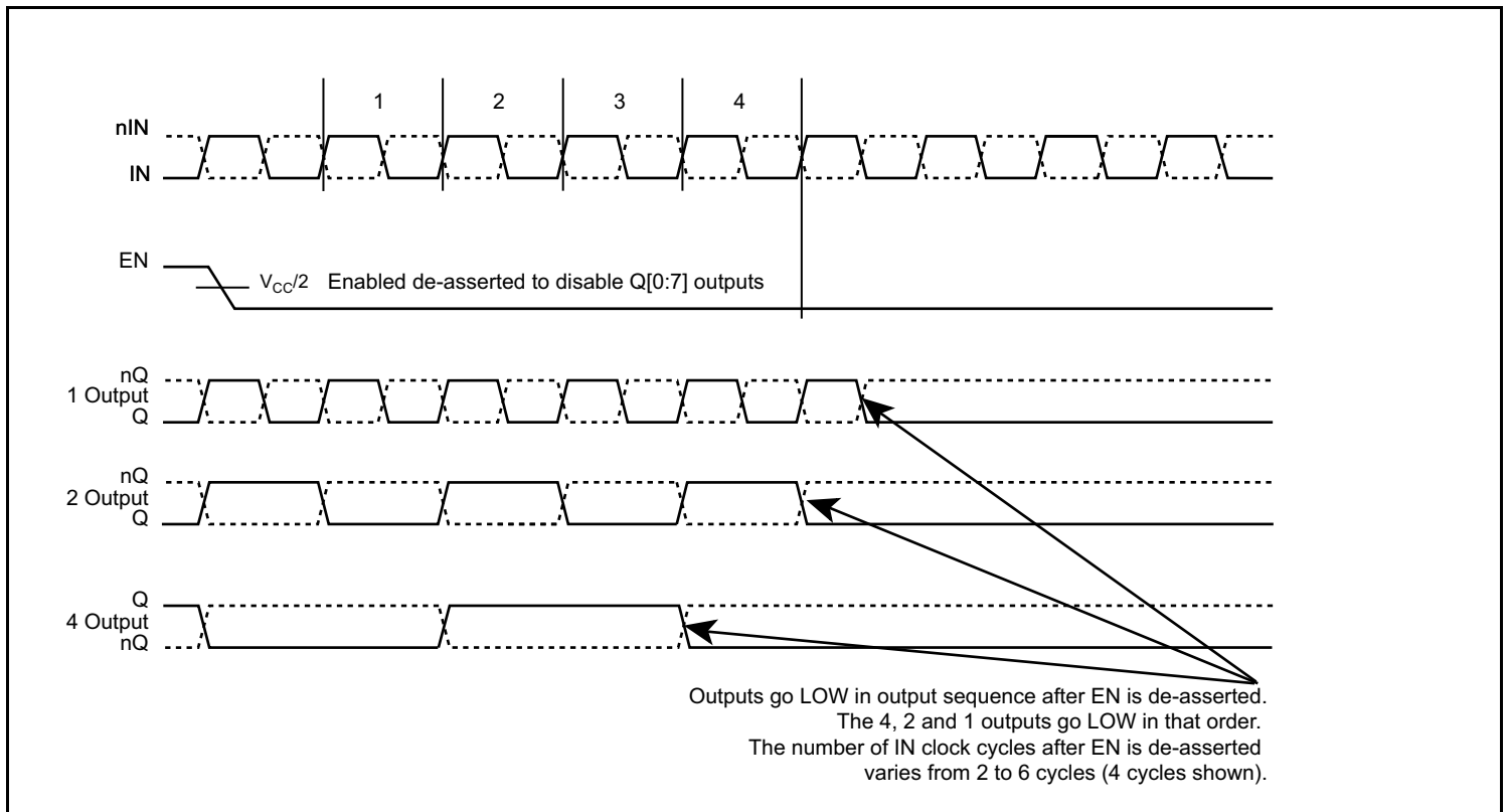
Figure 1C. Disabled Timing
