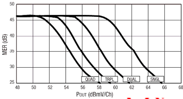
Figure 11. 64 QAM MER vs P_{out} Test Channel = 86 MHz, TX Channels= 75, 86, 93, 99 MHz
