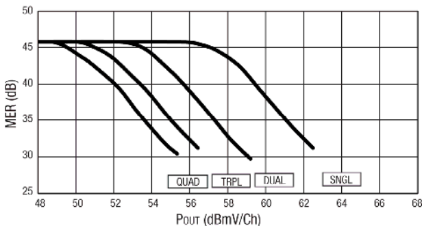
Figure 15. 256 QAM MER vs P_{out} Test Channel = 543 MHz, TX Channels= 537, 543, 549, 555 MHz
