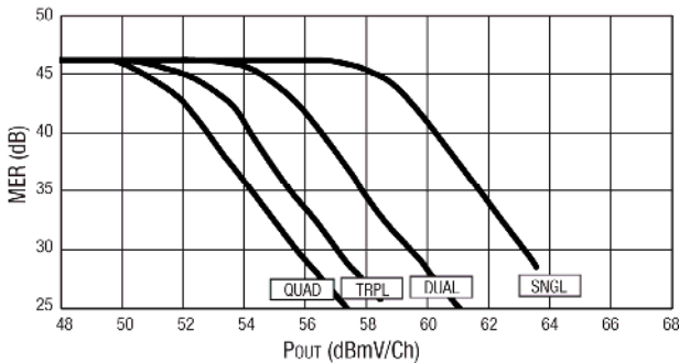
Figure 13. 64 QAM MER vs P_{out} Test Channel = 987 MHz, TX Channels= 981, 987, 993, 999 MHz
