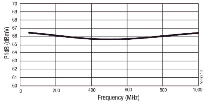
Figure 10. P1dB vs Frequency
