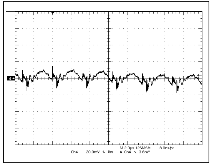
Fig-1.5V-5: Output voltage ripple (20mV/div.) for V_{out}=1.5V at full rated load current into a resistive load with external capacitance 47\mu F \times 2 ceramic + 1\mu F ceramic at V_{in}=12V .
