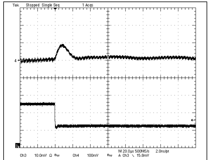
Fig-1.5V-7: Output voltage response for V_{out}=1.5V to negative load current step change from 5A to 2.5A with slew rate of -5A/\mu s at V_{in}=12V . C_o=47\mu F \times 2 ceramic.
