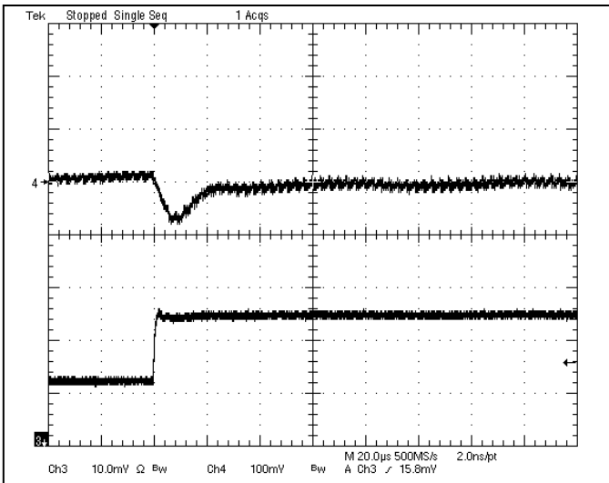
Fig-1.5V-6: Output voltage response for V_{out}=1.5V to positive load current step change from 2.5A to 5A with slew rate of 5A/\mu s at V_{in}=12V . C_o=47\mu F \times 2 ceramic.
