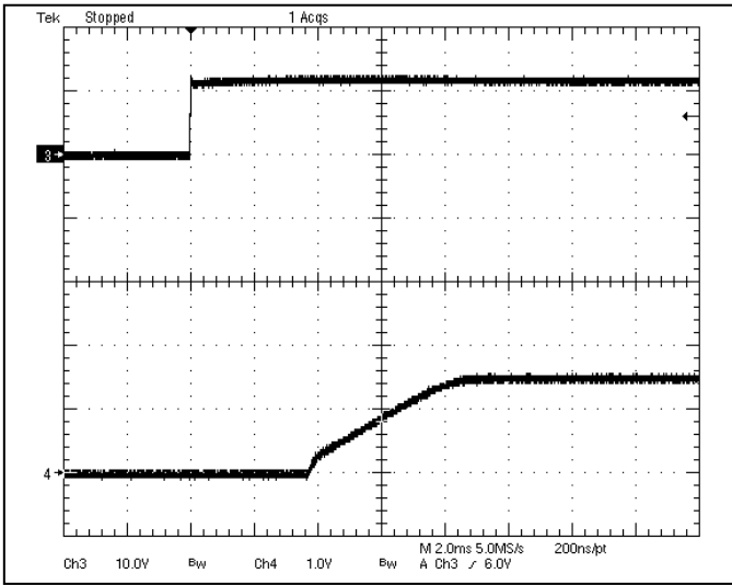
Fig-1.5V-4: Turn-on transient for V_{out}=1.5V with application of V_{in} at full rated load current (resistive) and 47\mu F \times 2 external capacitance at V_{in}=12V .
