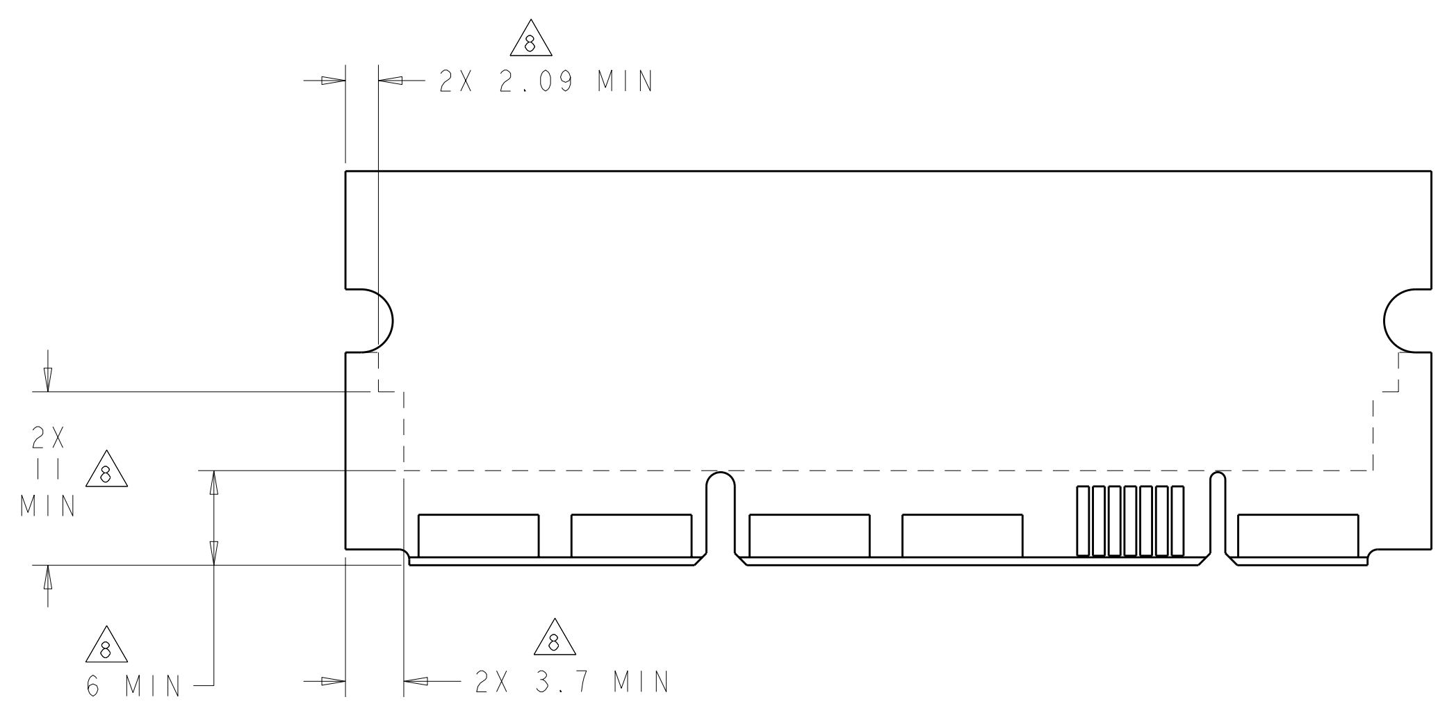
RCOMMENDED PC BOARD KEEP OUT AREA SCALE 3:1
