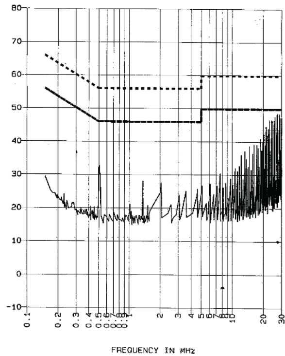
Figure 9. JW075A1 Conducted Noise with Filter 8-1387(F)
