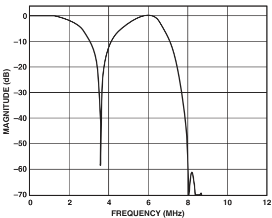
TPC 8. Luma NTSC Notch Filter
