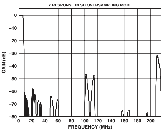
TPC 9. Y-16x Oversampling Filter
