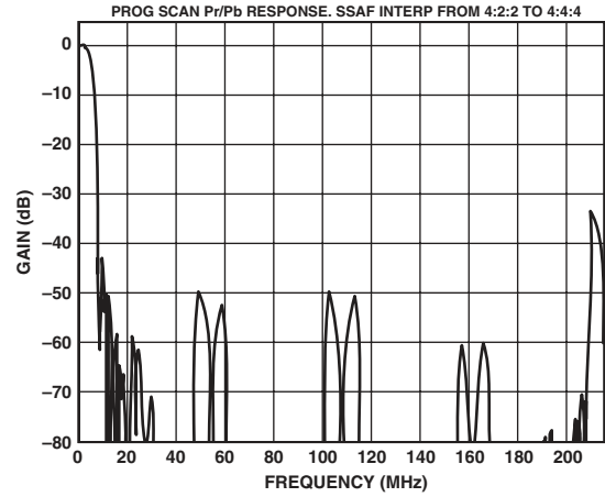
TPC 4. PS - UV 8x Oversampling Filter—SSAF
