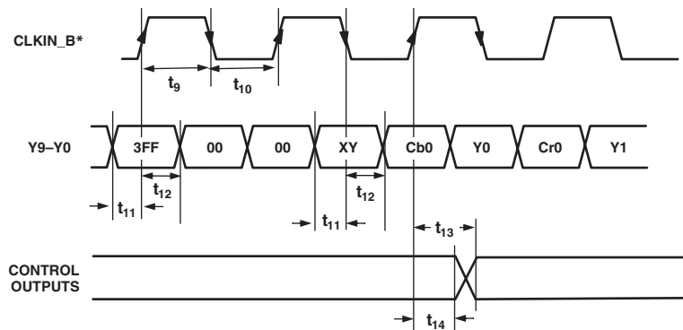
Figure 5. PS 4:2:2 1x10-Bit Interleaved at 54 MHz HSYNC/VSYNC Input Mode [Input Mode 111]
