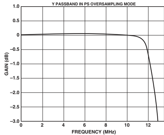
TPC 5. PS - Y 8x Oversampling Filter—Pass Band
