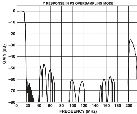
TPC 2. PS - Y 8x Oversampling Filter
