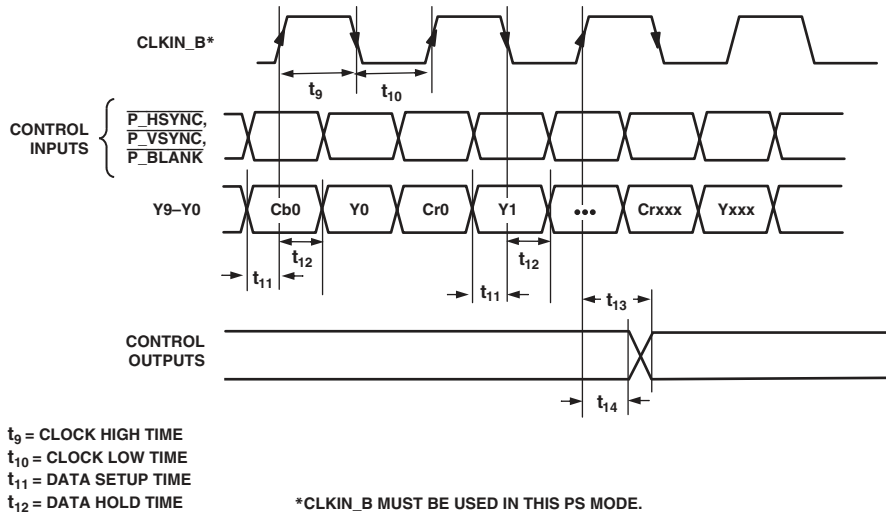
Figure 4. PS 4:2:2 1x10-Bit Interleaved at 27 MHz \overline{HSYNC}/\overline{VSYNC} Input Mode [Input Mode 100]
