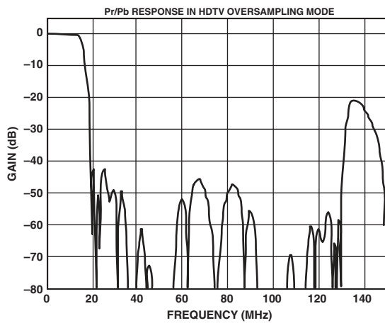
TPC 3. HDTV - UV 2x Oversampling Filter
