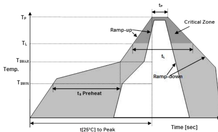
Reflow profile IPC/JEDEC J-STD-020 REV. C
