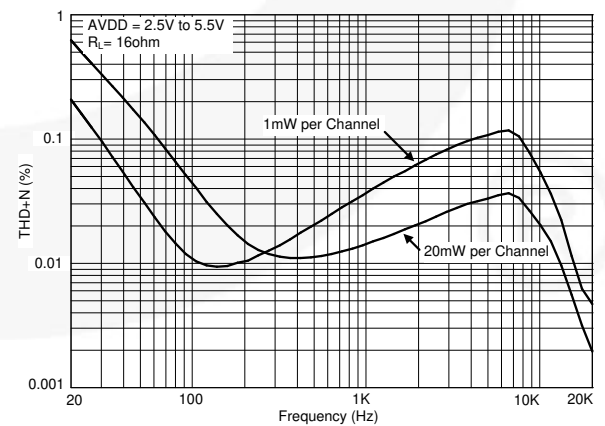
Figure 15. THD vs. Frequency at 16 \Omega
