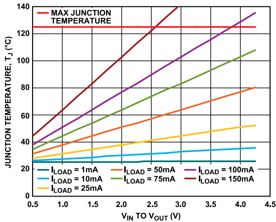
Figure 42. WLCSP, 0 mm 2 of PCB Copper, T A = 25°C
