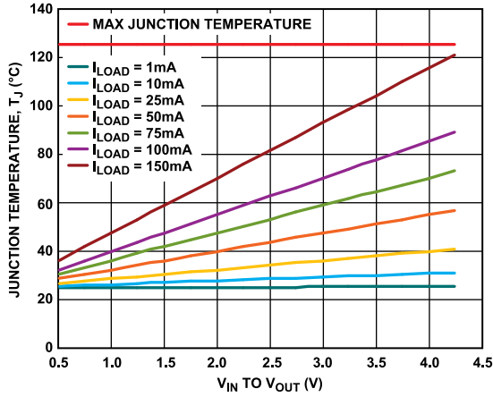
Figure 40. WLCSP, 500 mm 2 of PCB Copper, T A = 25°C
