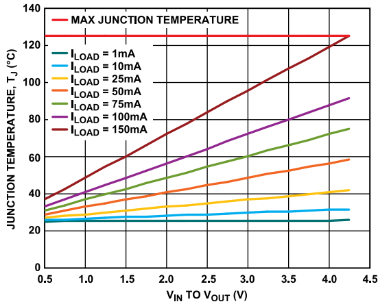
Figure 41. WLCSP, 100 mm 2 of PCB Copper, T A = 25°C
