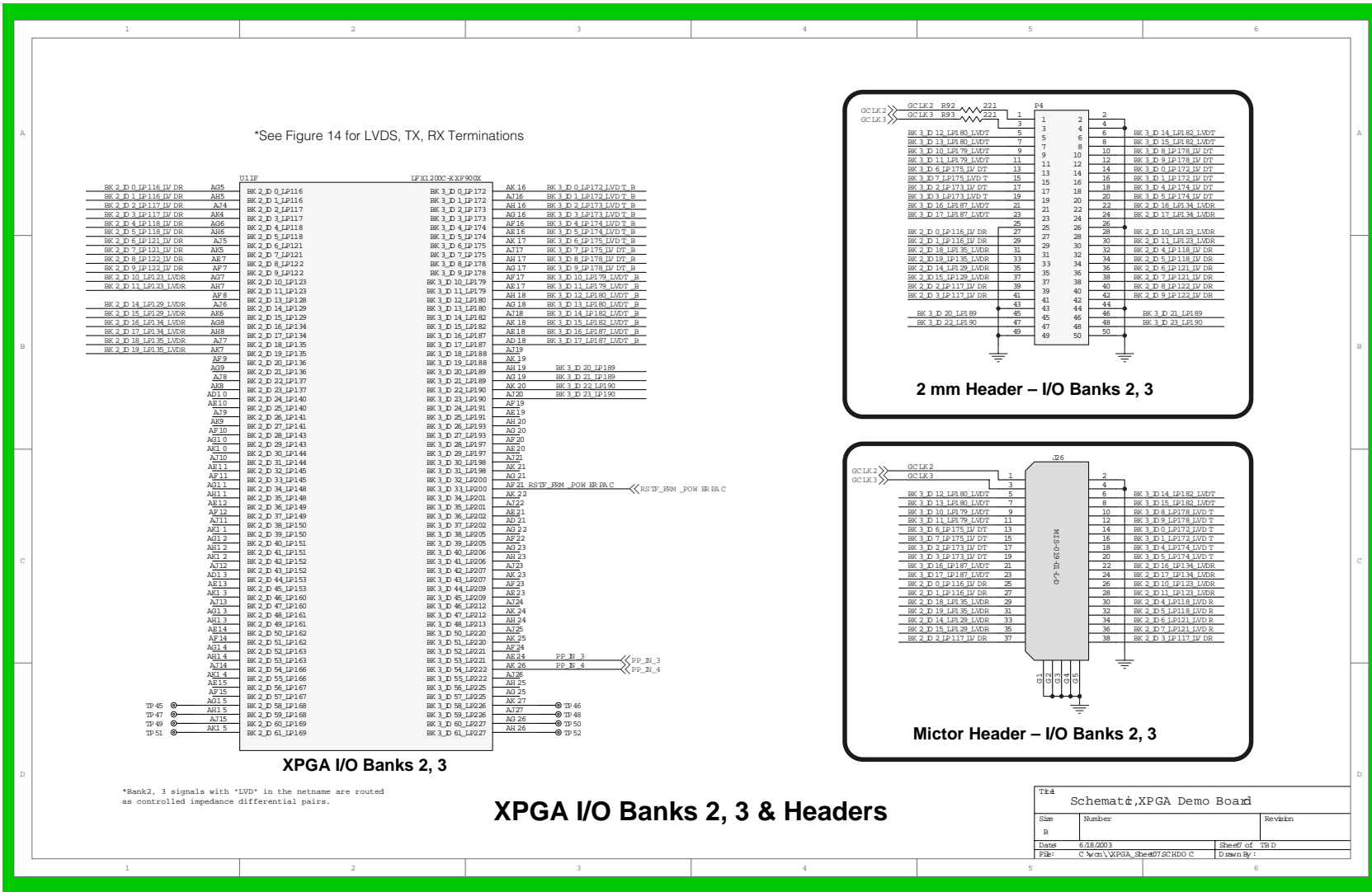
Figure 11. Lattice ispXPGA Evaluation Board Schematic
