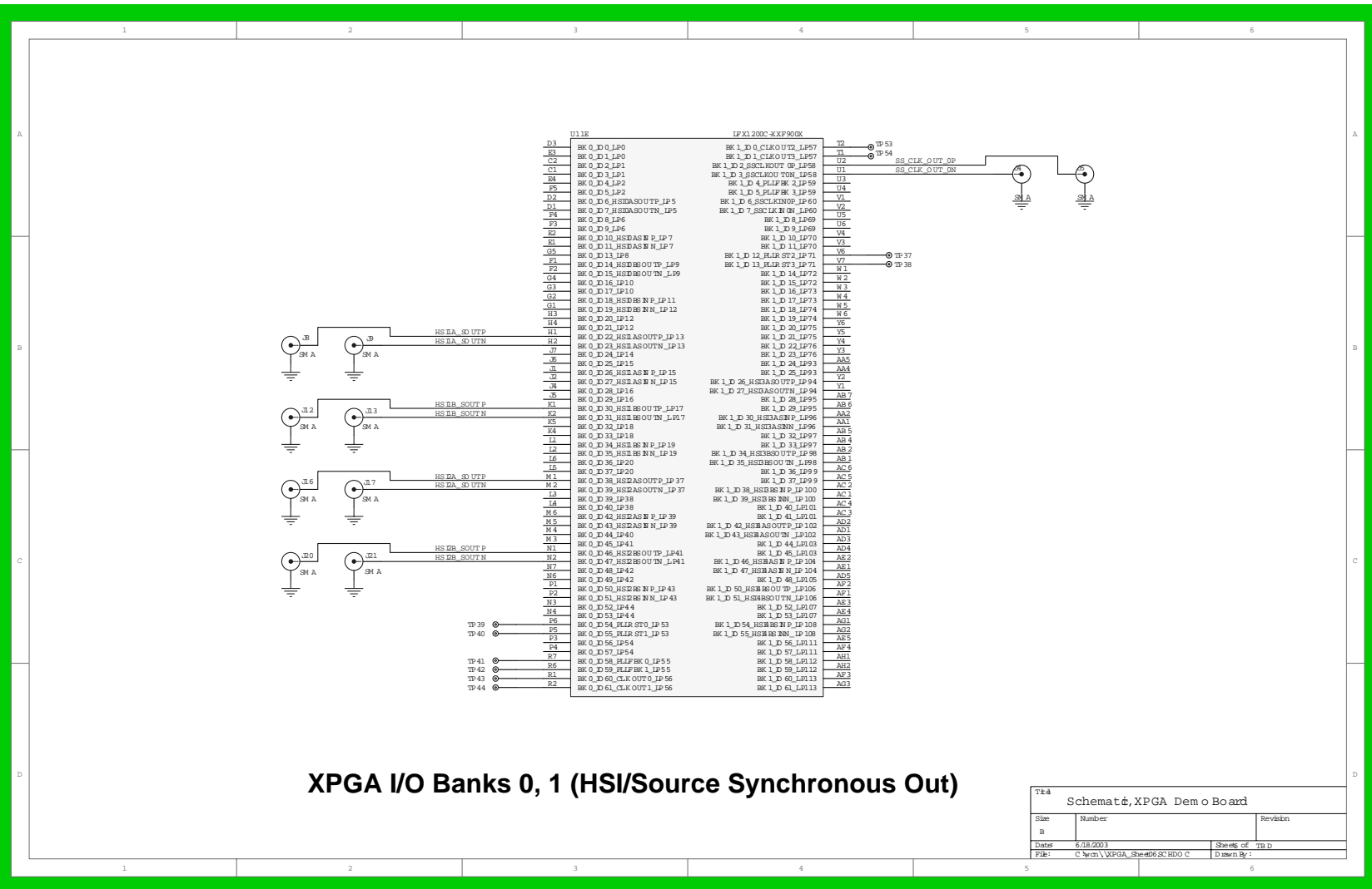
Figure 10. Lattice ispXPGA Evaluation Board Schematic
