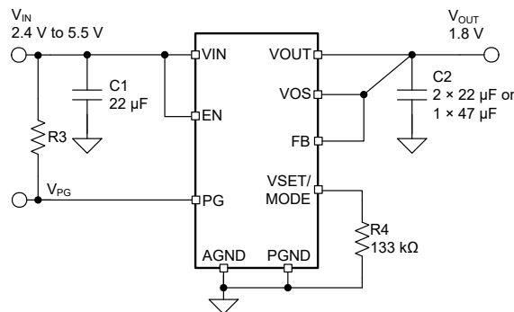
Figure 8-4. Fixed Output Voltage Application Circuit
