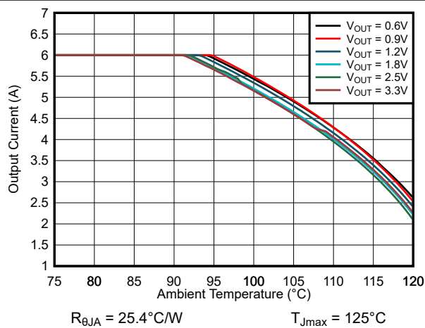
R_{\theta JA} = 25.4^\circ\text{C/W} T_{Jmax} = 125^\circ\text{C} Figure 9-30. Safe Operating Area V_{IN} = 5.0\text{-V} TPSM82866AA0HRDMR
