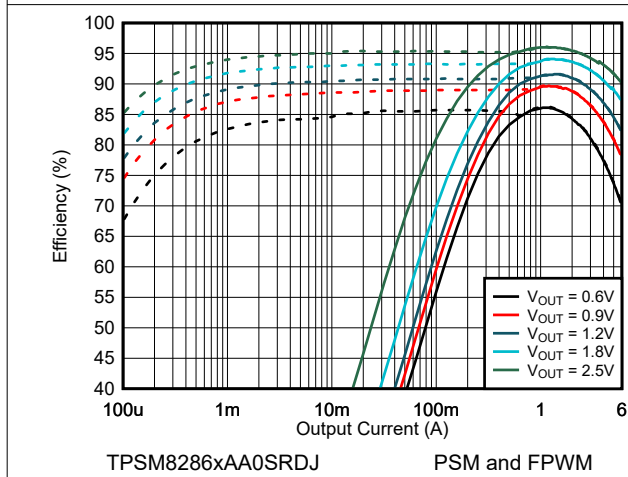
Figure 9-4. Efficiency V_{IN} = 3.3\text{ V} and T_A = 25^\circ\text{C}
