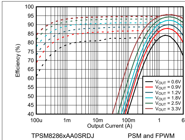
Figure 9-2. Efficiency V_{IN} = 5.0\text{ V} and T_A = 25^\circ\text{C}
