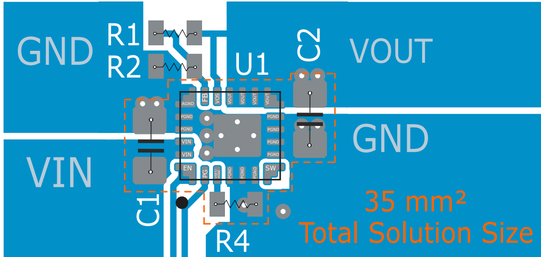
Figure 9-34. Layout Example
