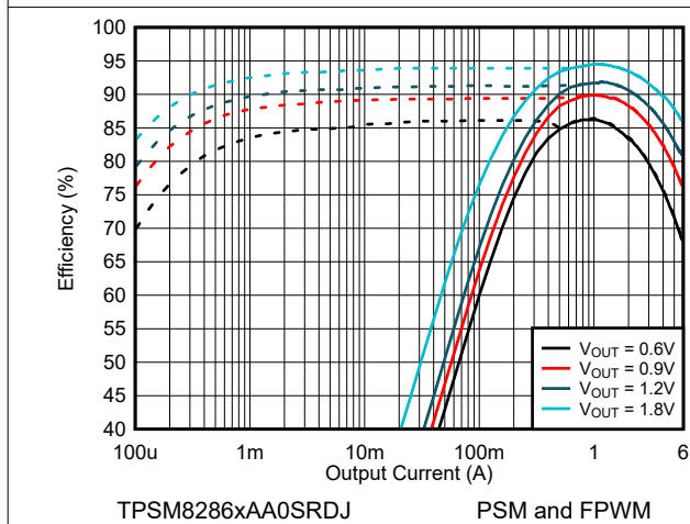
Figure 9-6. Efficiency V_{IN} = 2.8\text{ V} and T_A = 25^\circ\text{C}
