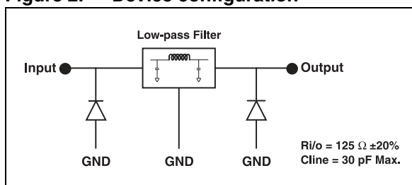
Figure 2. Device configuration
