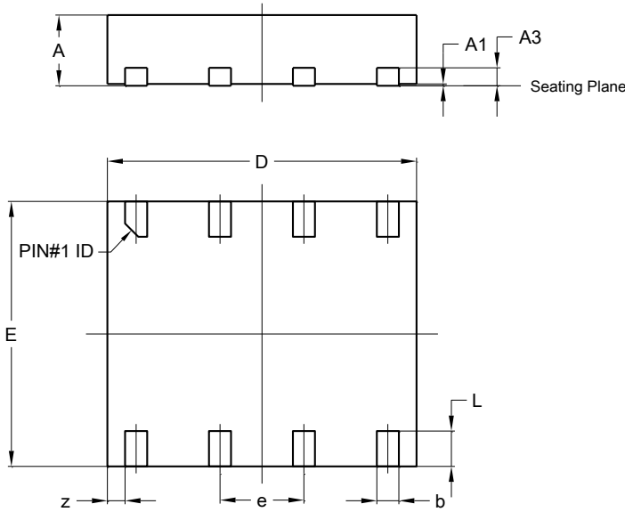
V-DFN3035-8
