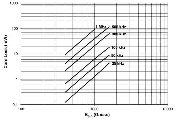
HCM1A0503-4R7-R
