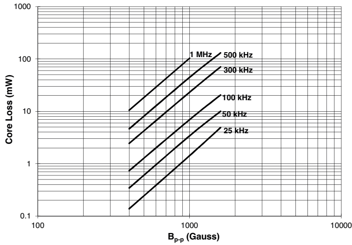
HCM1A0503-1R5-R
