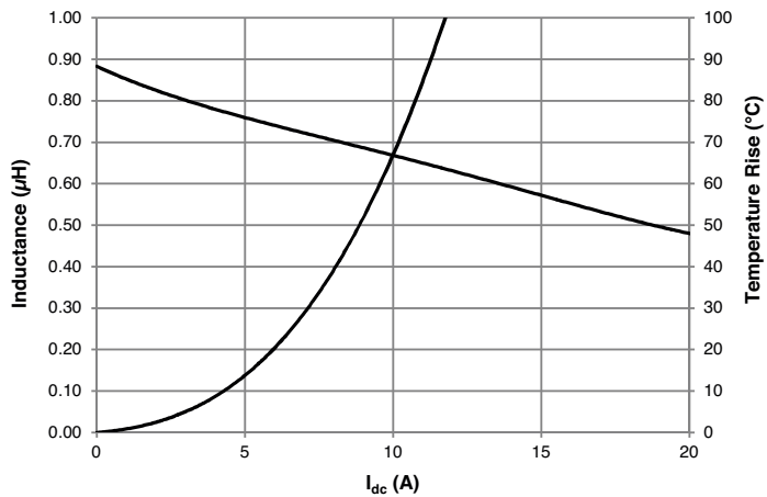
HCM1A0503-1R0-R
