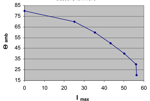
Max. allowable ambient Temp. at specific current (rms) B25667C4547A375
