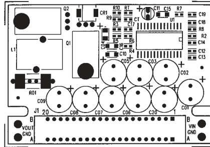
Figure 11. COMP Silkscreen
