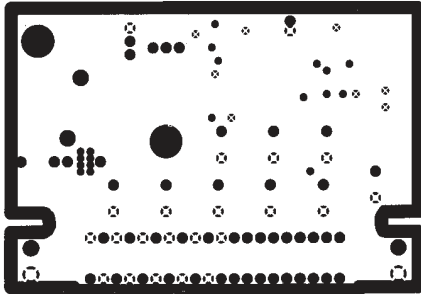
Figure 13. GND Layer
