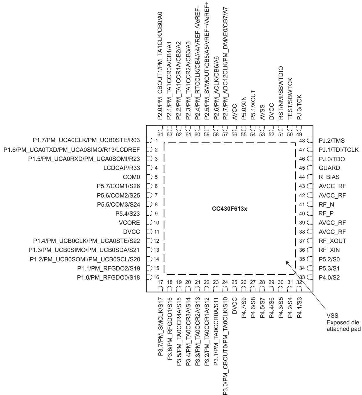
Figure 4-1. 64-Pin RGC Package (Top View), CC430F613x
