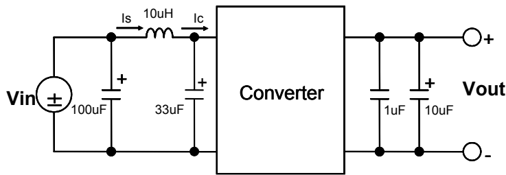
Fig.6.0V-8: Test Set-up for measuring input reflected ripple current.
