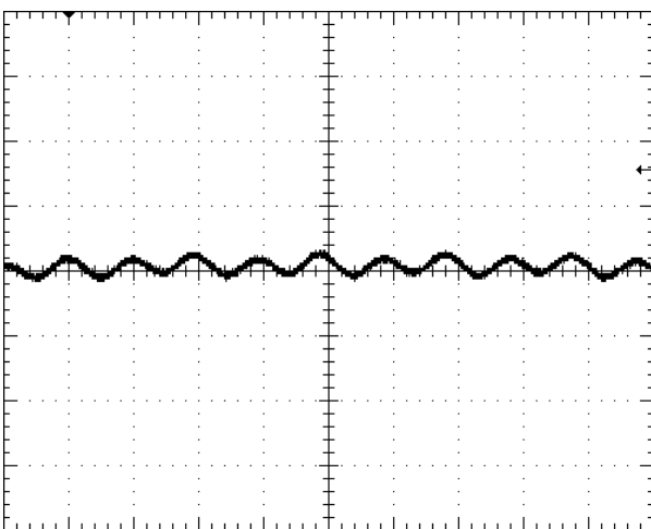
Fig.6.0V-9: Input reflected ripple current, I_s (10mA/div), measured through 10µH at the source at full rated load current and V_{in}=48V . Time scale: 2µs/div.
