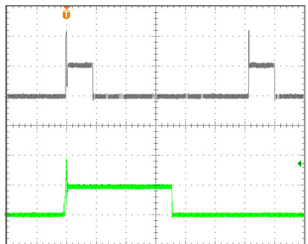
Fig.6.0V-12: Load current (top trace, 25A/div, 40ms/div) into a 10mΩ short circuit during restart, at V_{in} = 48V . Bottom trace (25A/div, 10ms/div) is an expansion of the top trace.
