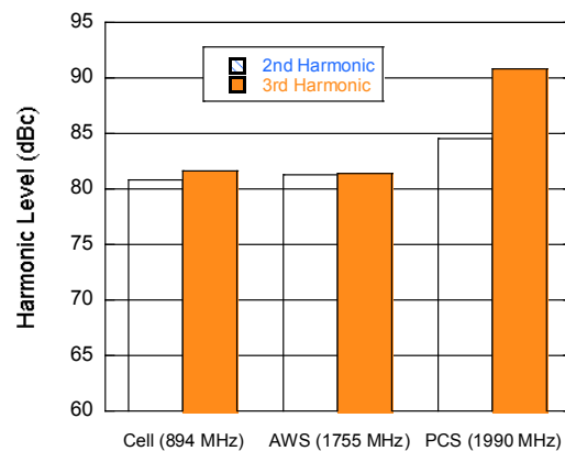
Harmonics
