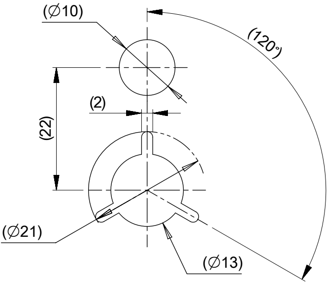
DETAIL "D"
