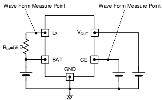
< Circuit No.⑤ >
