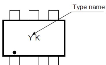
Fig. 8.1 Marking RN2910FE
