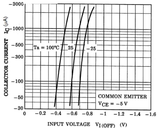
Fig. 9.4 RN2911EF I_C - V_{I(OFF)}
