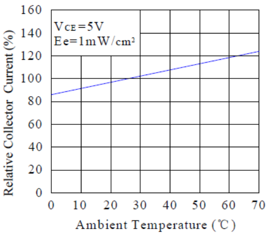
Relative Collector Current & Ambient Temperature
