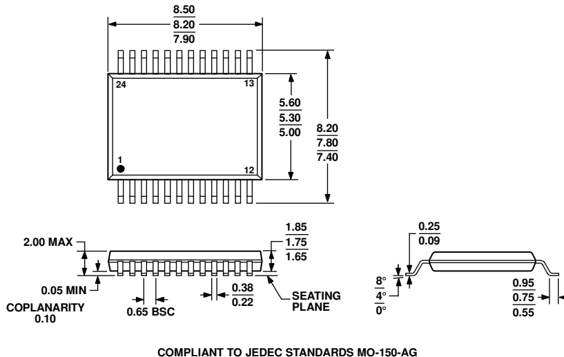
Figure 35. 24-Lead Shrink Small Outline Package [SSOP] (RS-24) Dimensions shown in millimeters
