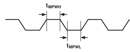
Figure 3. MCLK_IN Timing
