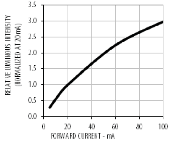
Figure 2 Luminous Intensity vs. Forward Current
