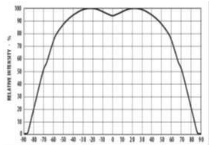
Figure 4 Radiation Pattern
