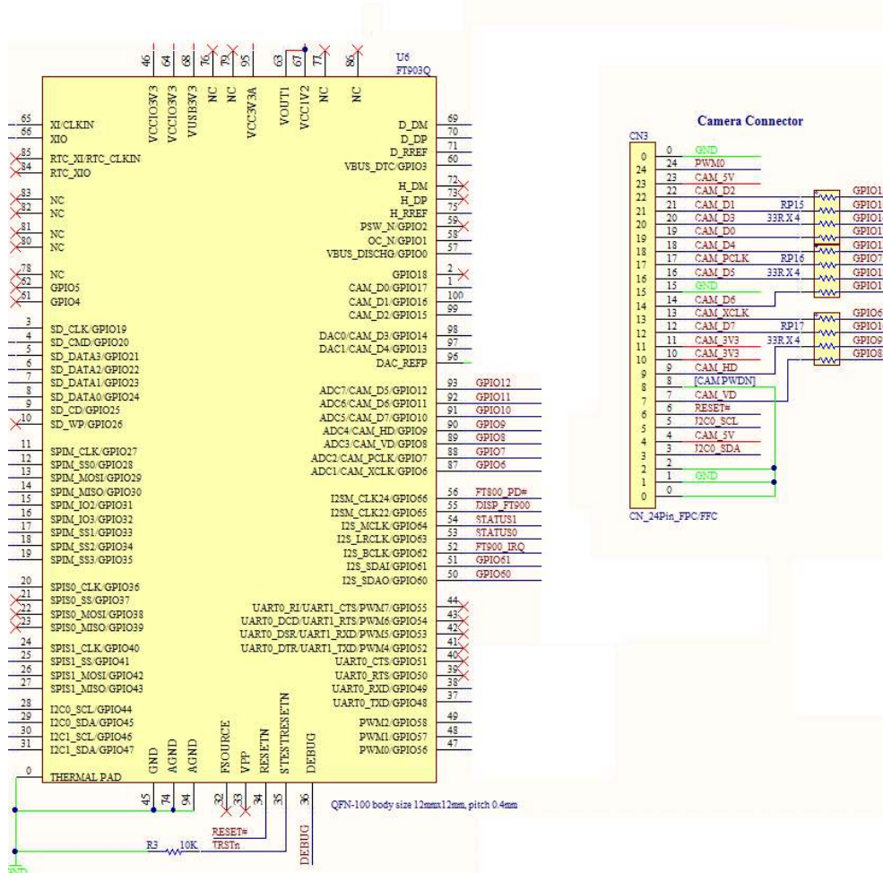
Figure 6 - Camera Interface
