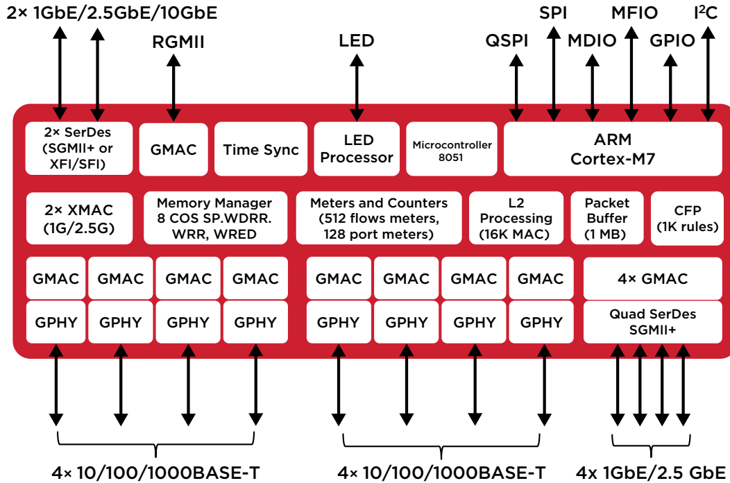
BCM5316X Block Diagram
