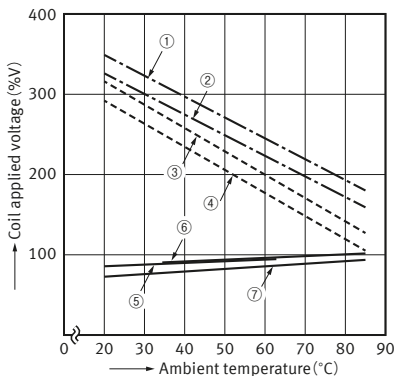
4-1. Ambient temperature characteristics ( 1 Form A )
