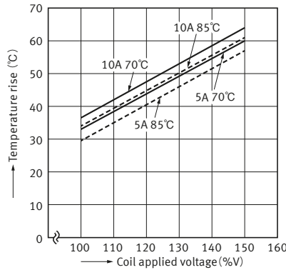
4-2. Ambient temperature characteristics ( 1 Form C )
