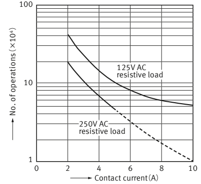
2. Switching life curve ( Form A contact )
