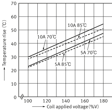
4-1. Ambient temperature characteristics ( 1 Form A )
