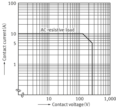
1-1. Max. switching capacity ( 1 Form A )
