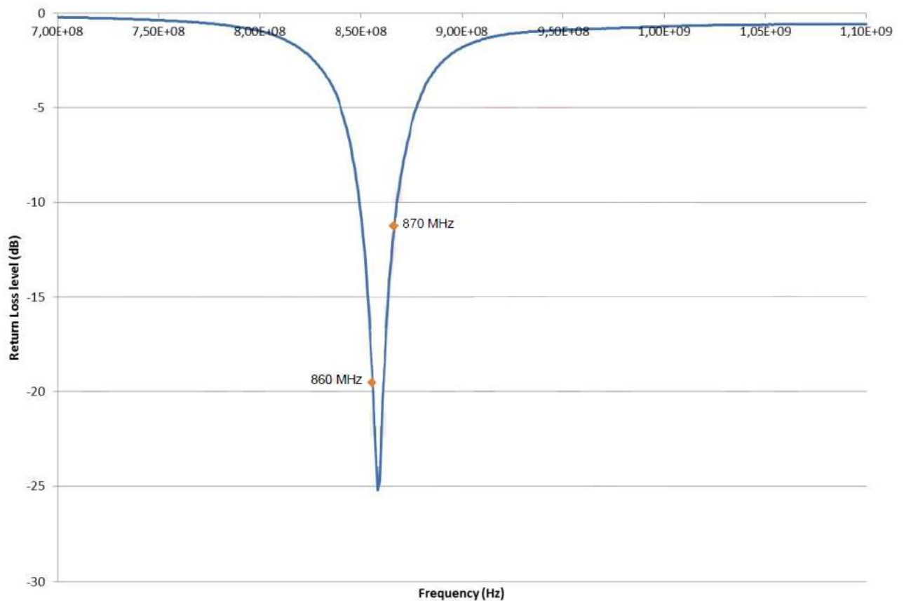
Return Loss
