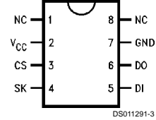
Alternate SO Pinout (TM8) NM93C14 Only
