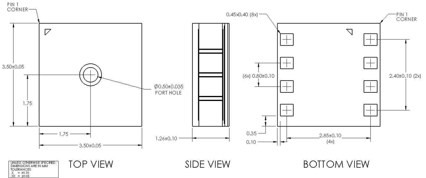
Figure 3. Package Dimensions
