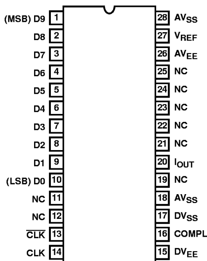
HI20201 (PDIP, SOIC) TOP VIEW
