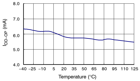
Figure 9. Operating Current
