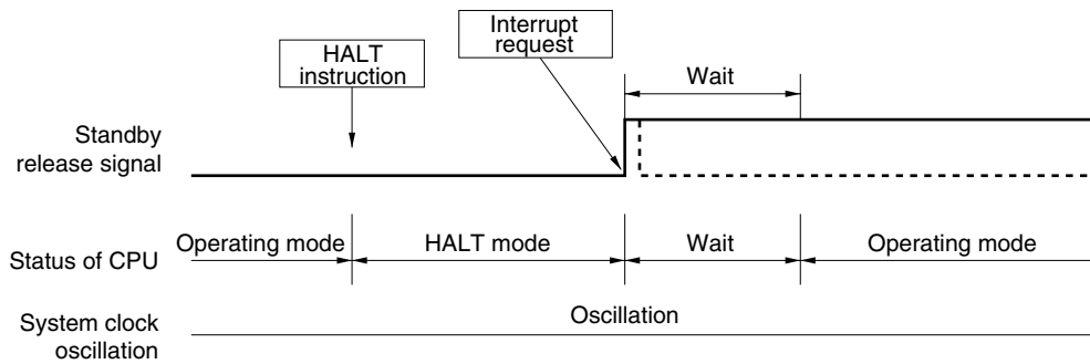
Figure 14-2. HALT Mode Release by Interrupt Request Generation
