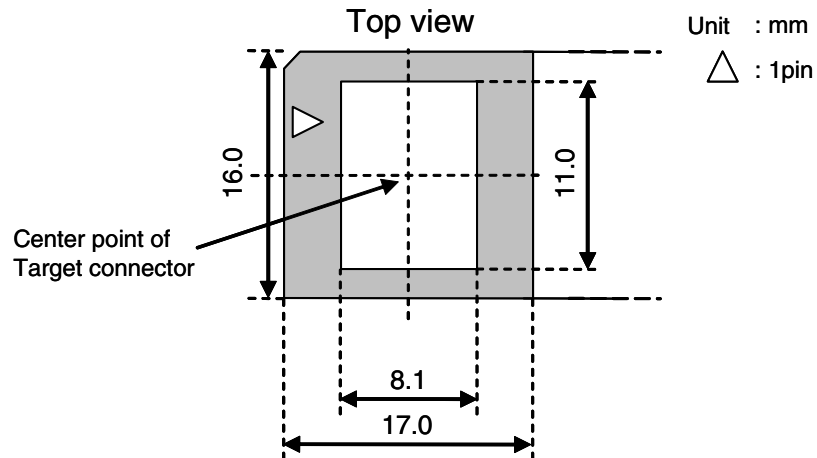
Figure B-1. When using the 78K0S/Kx1+ emulation probe (For 30-Pin MC Package)
