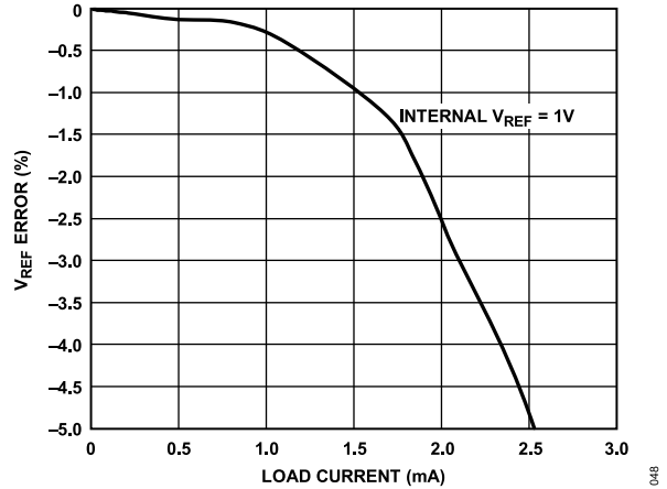
Figure 57. VREF Error vs. Load Current
