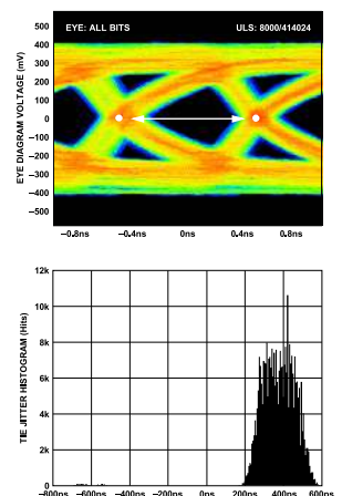
Figure 69. Data Eye for LVDS Outputs in ANSI-644 Mode with Trace Lengths Greater Than 24 Inches on Standard FR-4 Material, External 100 Ω Far-End Termination Only
