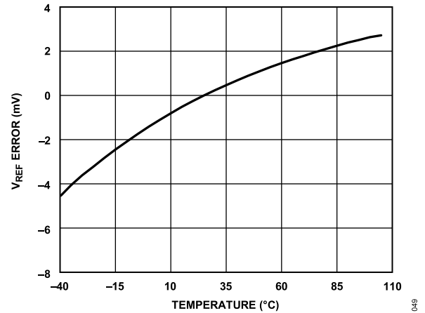
Figure 58. Typical VREF Drift
