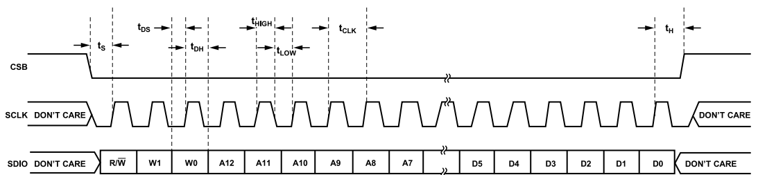
Figure 70. Serial Port Interface Timing Diagram
