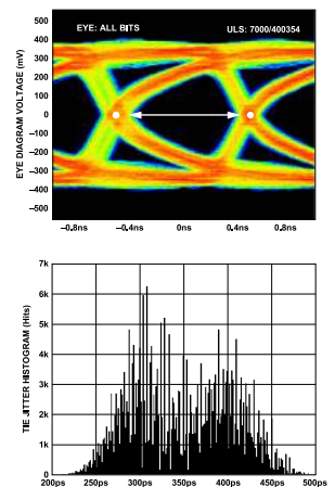
Figure 68. Data Eye for LVDS Outputs in ANSI-644 Mode with Trace Lengths of Less Than 24 Inches on Standard FR-4 Material, External 100 Ω Far-End Termination Only
