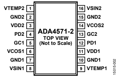
Figure 2. Pin Configuration
