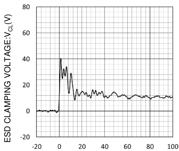
TIME(ns) ESD CLAMPING VOLTAGE (IEC61000-4-2 +8kV CONTACT)
